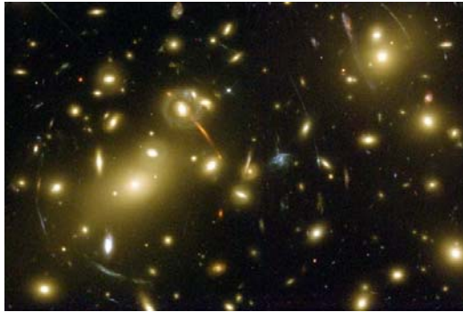
Fig. 1. Abell 2218: A Galaxy Cluster Lens [1].
