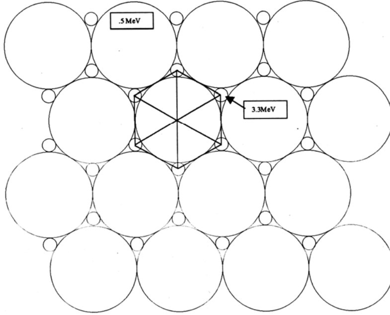
Fig. 1. Hexagonal configuration of a two dimensional slice through the Spin Matrix. If we take the larger areas to be 0.511 MeV, then the smaller areas shown, geometrically come out to be ~3.3 MeV.
