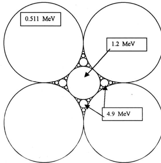
Fig. 3. Quad Spin Matrix configuration.
